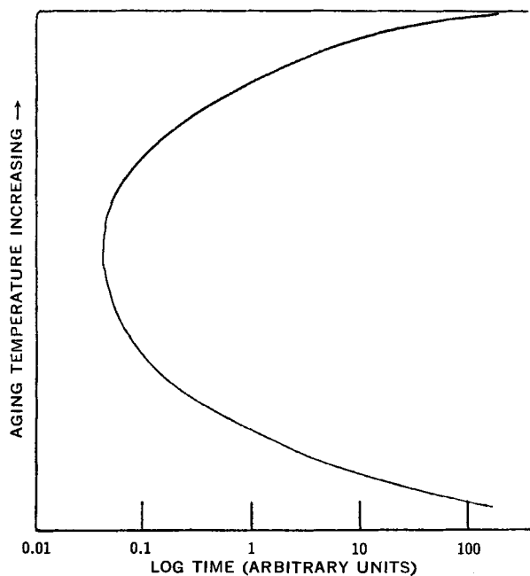
Figure 18—Diagram illustrating the time for 100% of precipitation from a supersaturated solid solution as a function of aging temperature (from Reference 54, p. 240, reprinted with permission).
