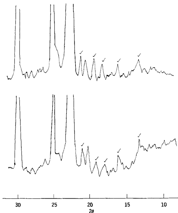
Figure 4—X-ray diffraction spectra of a physical mixture of 10% chloramphenicol-90% urea (bottom) and resolidified fused mixture of 10% chloramphenicol-90% urea (top). Arrows indicate diffraction peaks due to the presence of chloramphenicol crystallites.
