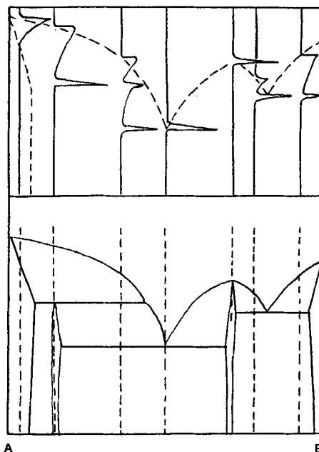
Figure 11—Typical DTA thermograms corresponding to a hypothetical binary system (from Reference 52, reprinted with permission).
