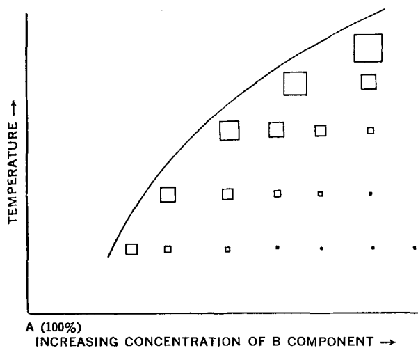
Figure 16 —Diagram illustrating relative nuclei and particle size of precipitation from supersaturated solid solutions at various temperatures and compositions (from Reference 55, p. 398, reprinted with permission).
