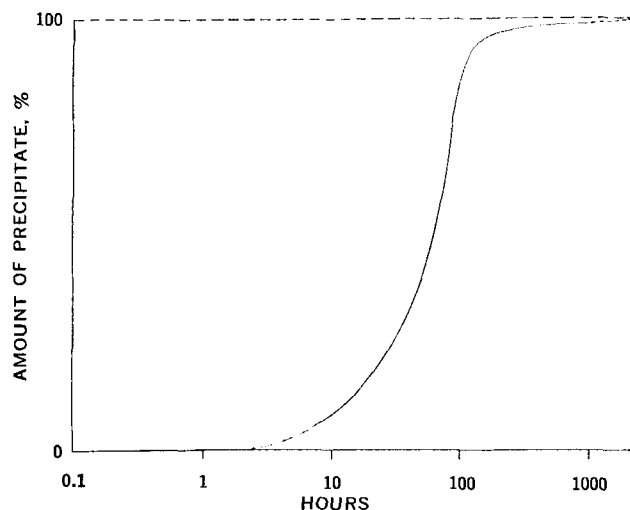
Figure 17 —Amount of precipitate as a function of time in an iron-carbon alloy (0.018% carbon) allowed to precipitate from a supersaturated solution at 76° (from Reference 54, p. 239, reprinted with permission).
