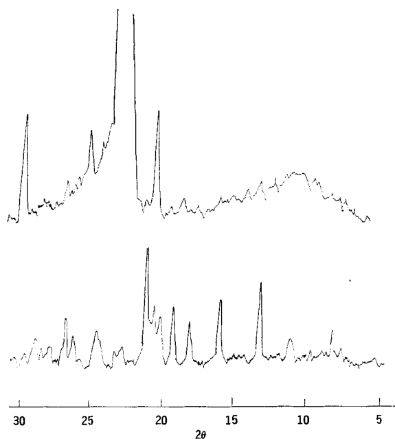
Figure 3—X-ray diffraction spectra of pure chloramphenicol (bottom) and pure urea (top).
