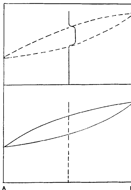
Figure 12—A DTA thermogram of a continuous solid solution system (from Reference 52, reprinted with permission).
