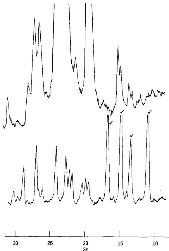
Figure 8—X-ray diffraction spectra of pure griseofulvin (bottom) and pure polyethylene glycol 6000 powders (top).
