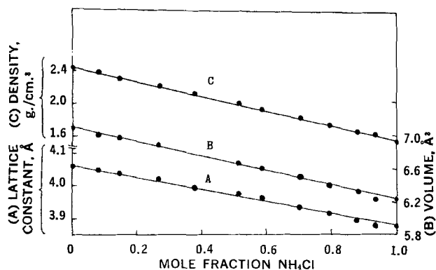
Figure 13 —Variation of composition of continuous solid solution of \text{NH}_4\text{Cl} - \text{NH}_4\text{Br} system with: (A) lattice constant, Å; (B) unit cell volume, Å 3 ; and (C) density, g./cm. 3 ; low temperature, high-angle data only (from Reference 125, Fig. 3, reprinted with permission).
